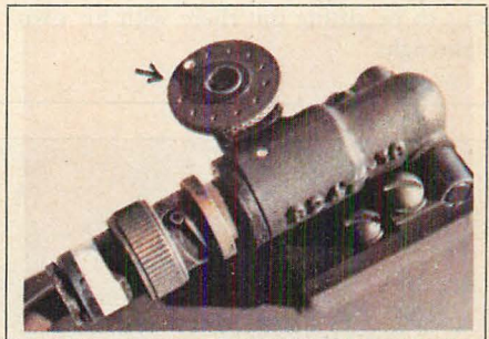
Aiming reticle in this infrared sight consists of small vertical bar of light, which can be varied in intensity, projected onto lens. Vertical adjustment for sighting-in is made easy by merely turning dial to move bar up or down. Tiny projector bulb is used as light source and has 1000-hr. service life.
